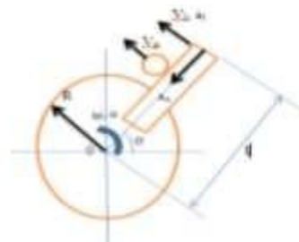
Fig. 3. A rotor bar of a hammer crusher
